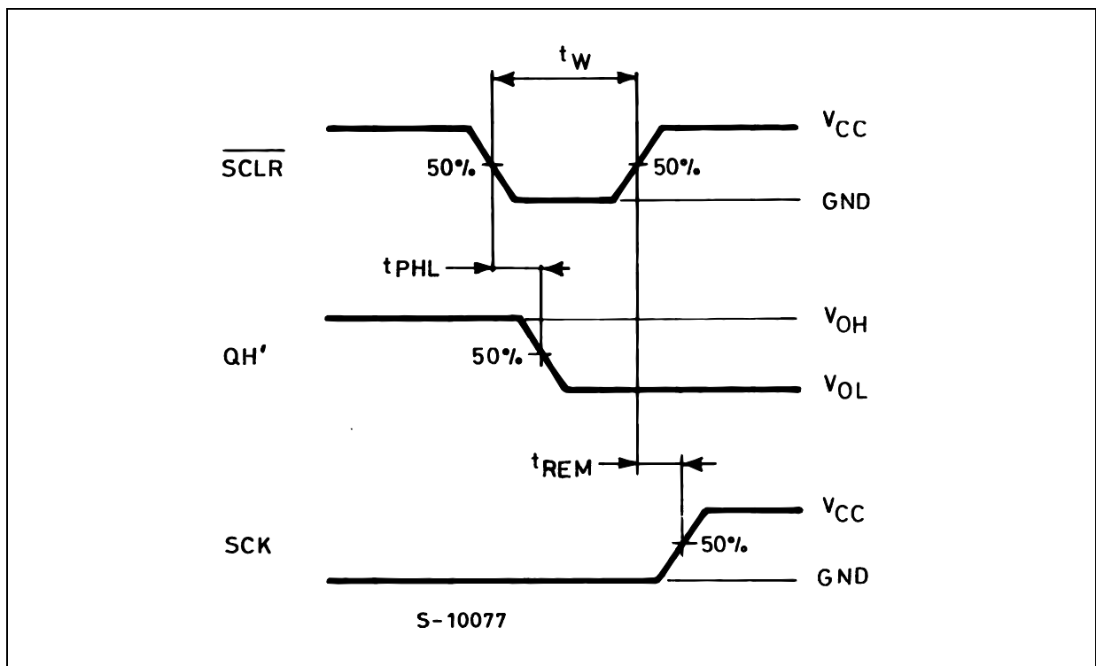
WAVEFORM 3 : MINIMUM PULSE WIDTH AND REMOVAL TIME ( f=1\text{MHz} ; 50% duty cycle)
